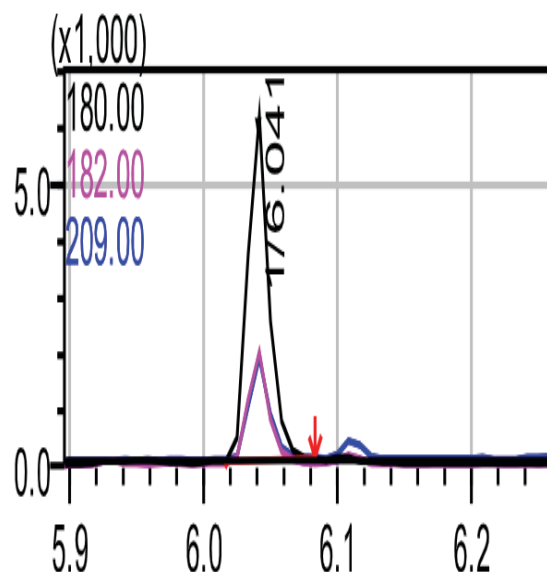
Figure 8- RT, m/z ratio, and reference ions for Ketamine.
